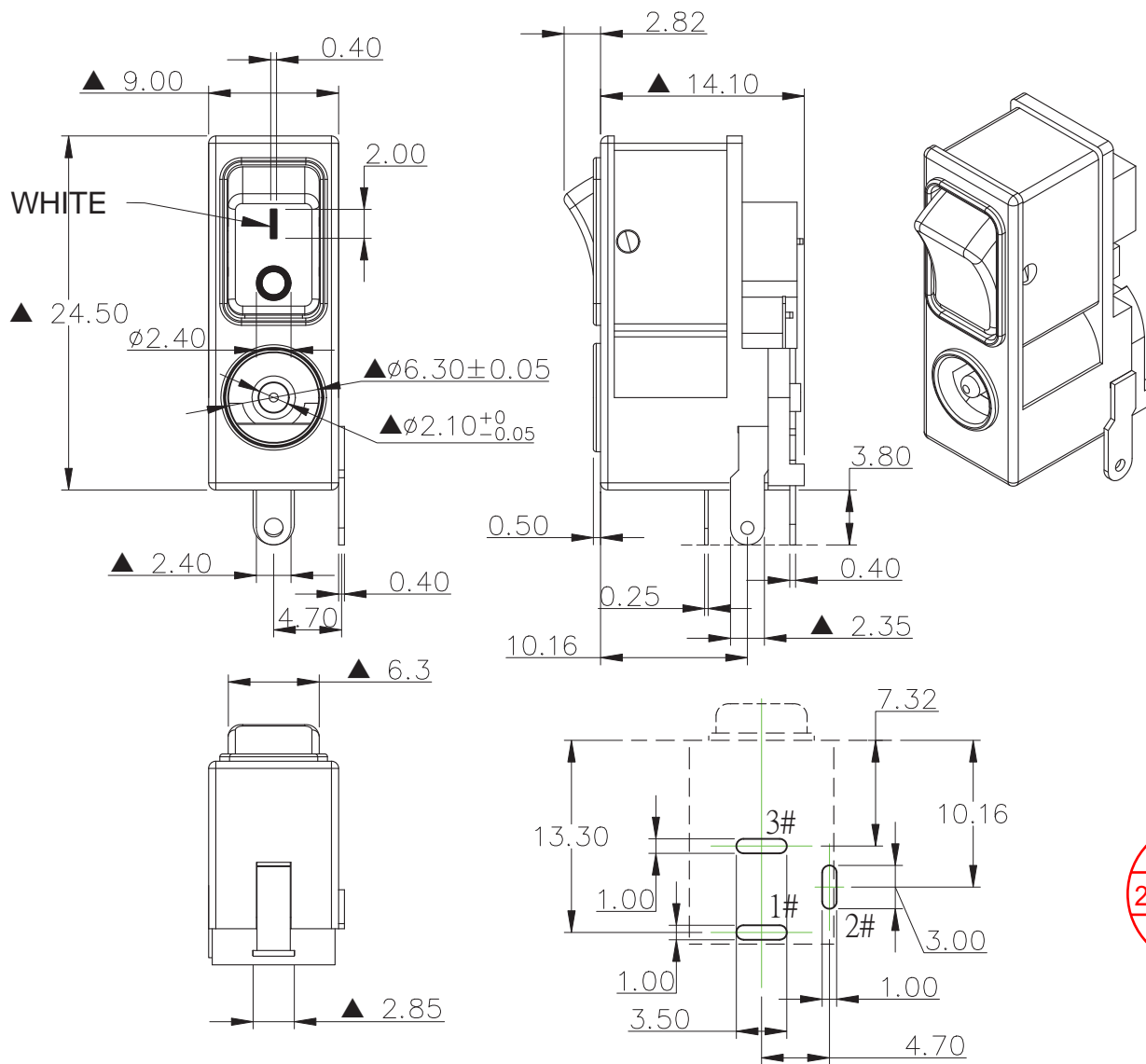
P. C. B LAYOUT BOTTOM VIEW
